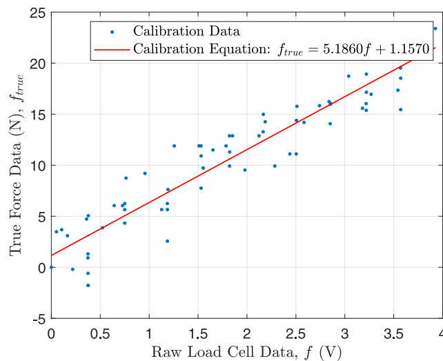
Fig 5. The load cell was calibrated by fitting the linear relationship to the raw voltage from the load cell to the expected force produced by stretching a spring with a known rate constant. The noise in the “true force data” is a result of the low resolution of the ultrasonic displacement sensor.
