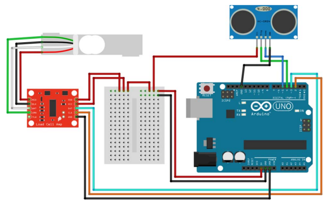
Fig 4. Wiring diagram for the load cell (top left), ultrasound displacement sensor (top right), and Arduino Uno microcontroller. The load cell requires the use of a signal amplifier (left) to increase the output voltage prior to being recorded by the microcontroller. Both sensors run off the Arduino Uno onboard 5-V power supply.
