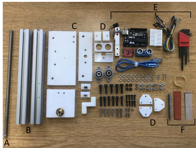
Fig 2. The lab kits are given to students disassembled. Each kit consists of the (A) leadscrew, (B) frame and hardware, (C) custom end blocks, (D) 3D printed parts, (E) electronics and sensors, and (F) test specimens to conduct a series of 3 separate lab activities exploring concepts pertaining to elasticity and viscoelasticity.
