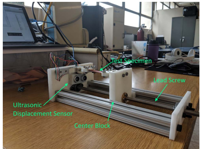
Fig 3. The fully assembled desktop tensile testing system connects to a laptop or desktop computer through the Arduino USB interface. A MATLAB script is used to record the measurement data collected by Arduino. When the leadscrew is turned, the center block travels horizontally.
