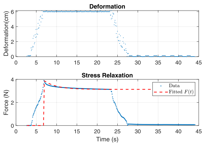
Fig 6. Sample deformation and force plots for the stress and relaxation testing of the silicone rubber specimen. The sample was quickly stretched to a 5.9-cm deformation, held at a constant length for approximately 16 s, and then returned to the original length. The SLS material constants were then determined by performing an exponential linear regression on the decaying force versus time data. This analysis returned parameters E_1 = 57.9 N/m, E_2 = 14.4 N/m, and \tau = 2.0 s -1 .
