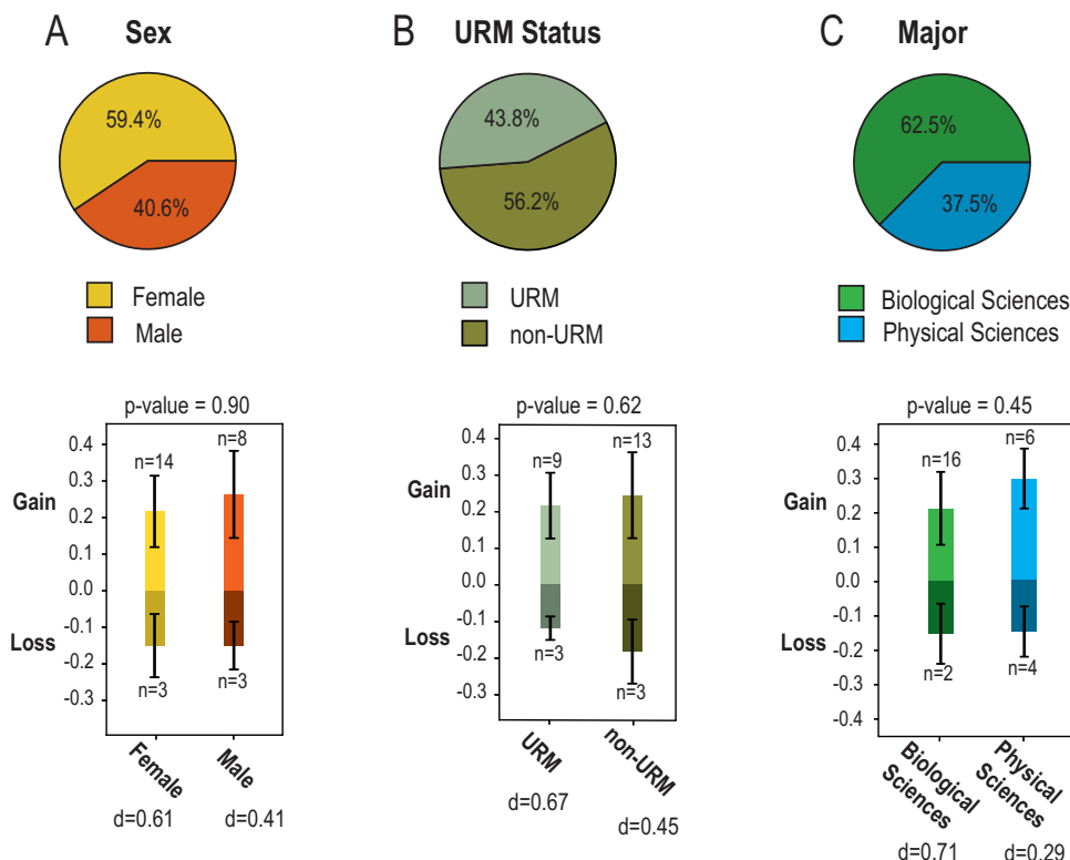
Fig 4. The BCIS shows no bias for sex or URM. Pie charts show the distribution of student demographics based on (A) sex, (B) URM status, and (C) college major. Bar charts show the mean of the gain (positive) and loss (negative), with the error bars denoting the standard deviation for each distribution. The effect size ( d ) is shown below each demographic. Sample size for each group is denoted by “ n ” near the error bar for that group. The 4 students with no change are not shown in the bar charts.
